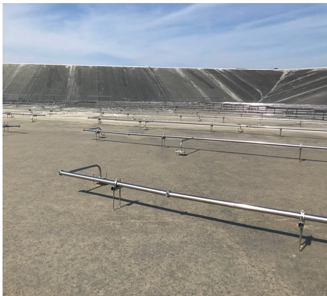
BioMix nozzles installed at the floor of each tank provide uniform mixing over a wide range of operating water levels.
